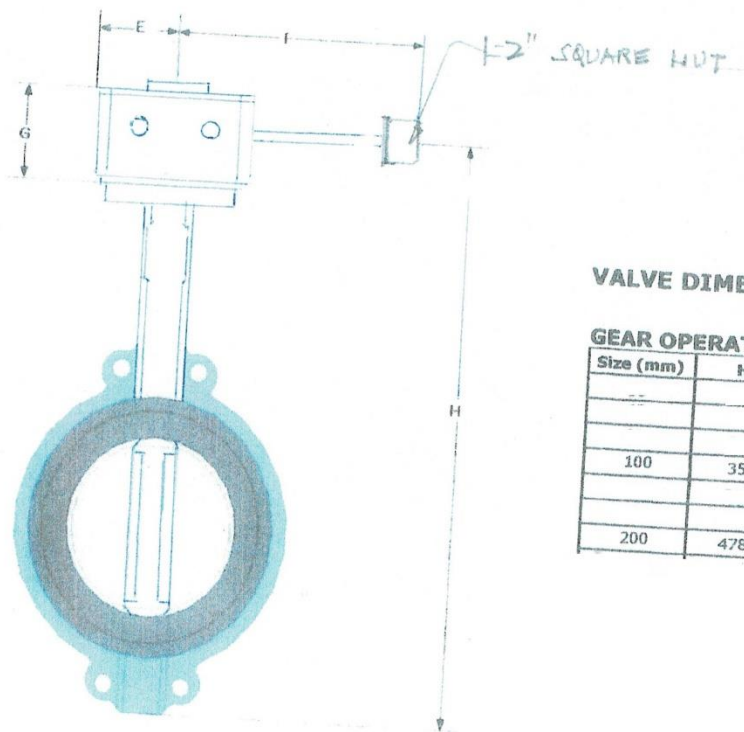
BUTTERFLY VALVE GEAR OPERATOR (WAFER TYPE)
