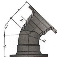
C.I. Bend Mechanical Type 45 Degree
