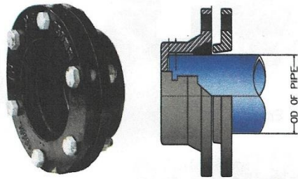
CI Mechanical Cap Plug
