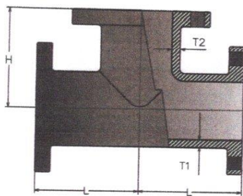
C.I. Tee Flange Type
