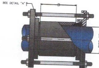
C.I. Sleeve Type Coupling for PVC Pipe
