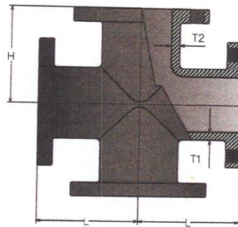
C.I. Cross Tee Flange Type
