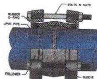
SECTION C.I. Gibault Joint for PVC
